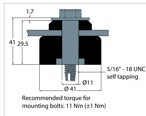
Mounting grommet
